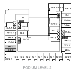
PODIUM LEVEL 2
