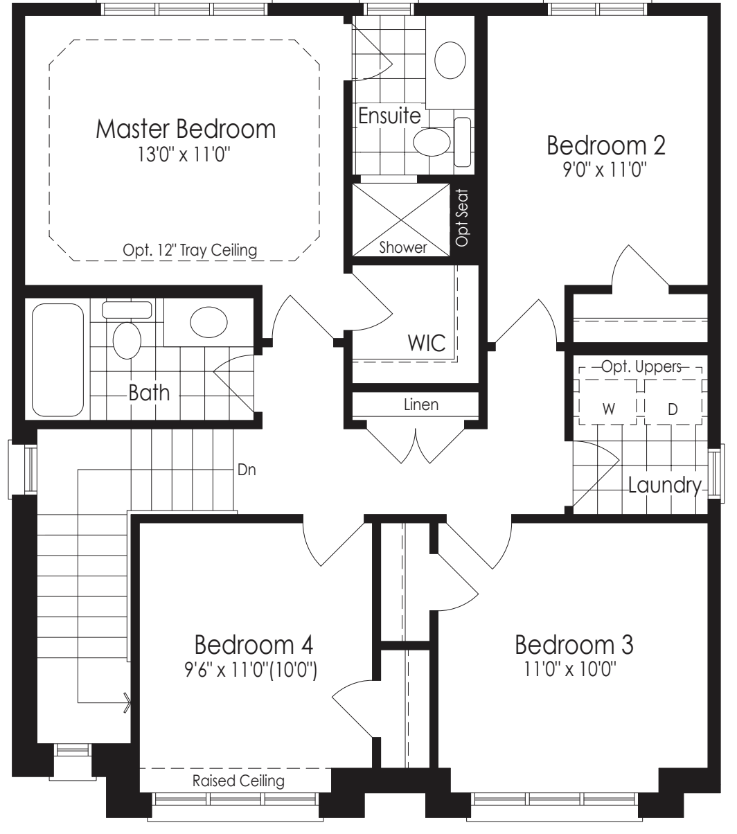
Second Floor Elev. A & B
