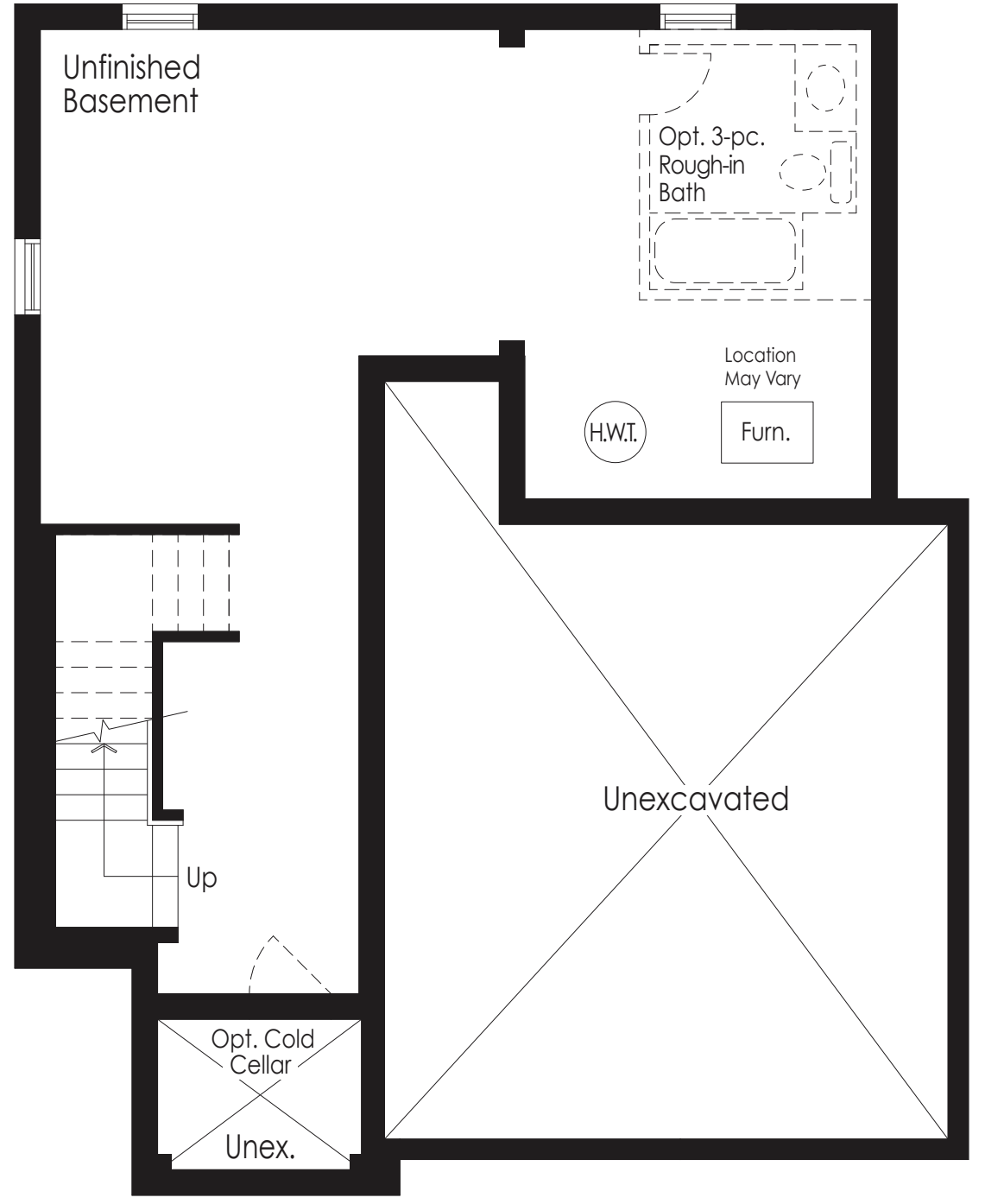
Basement Elev. A & B
