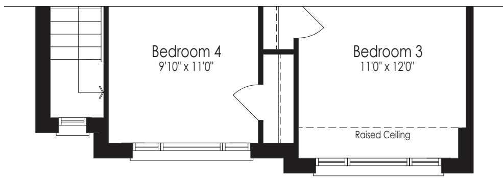
Second Floor Elev. C
