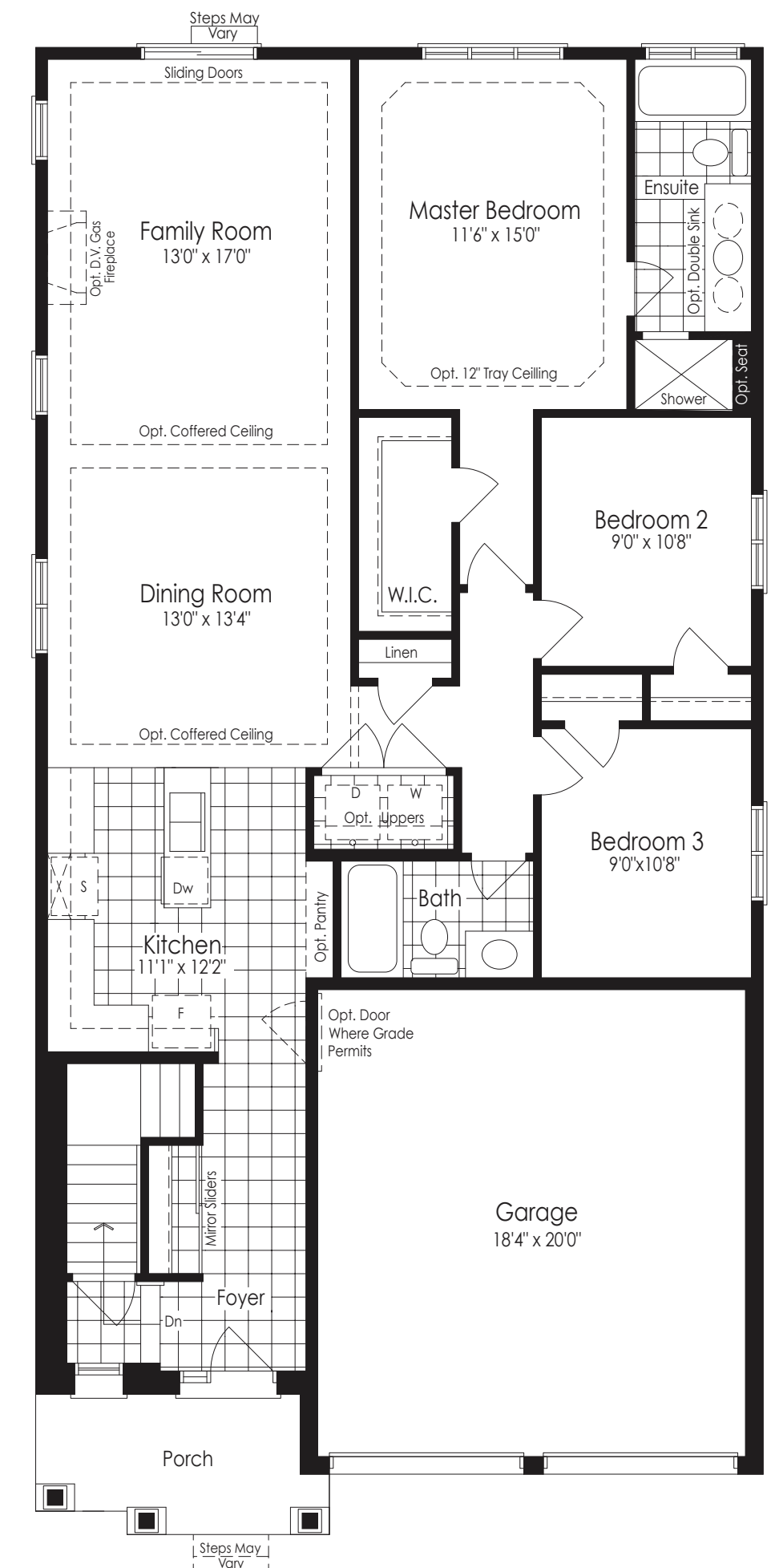
Ground Floor Elev. A
