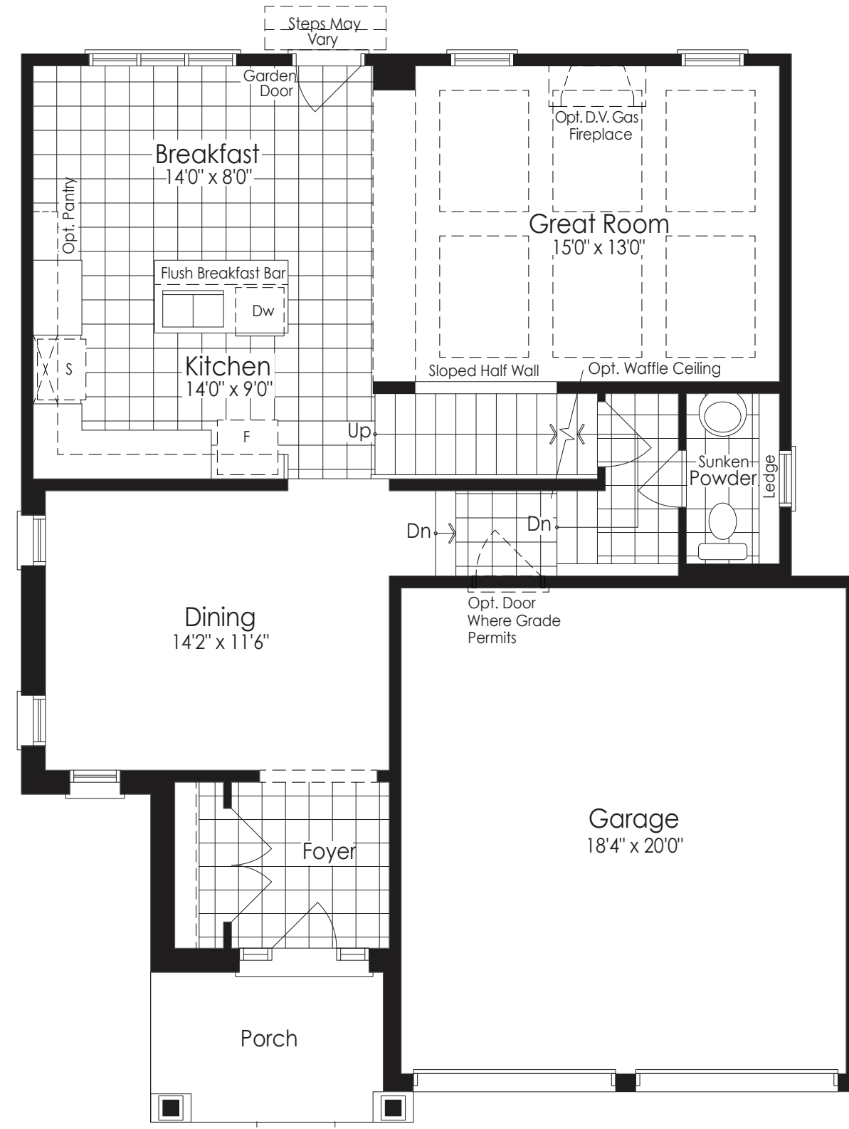
Ground Floor Elev. A & B
