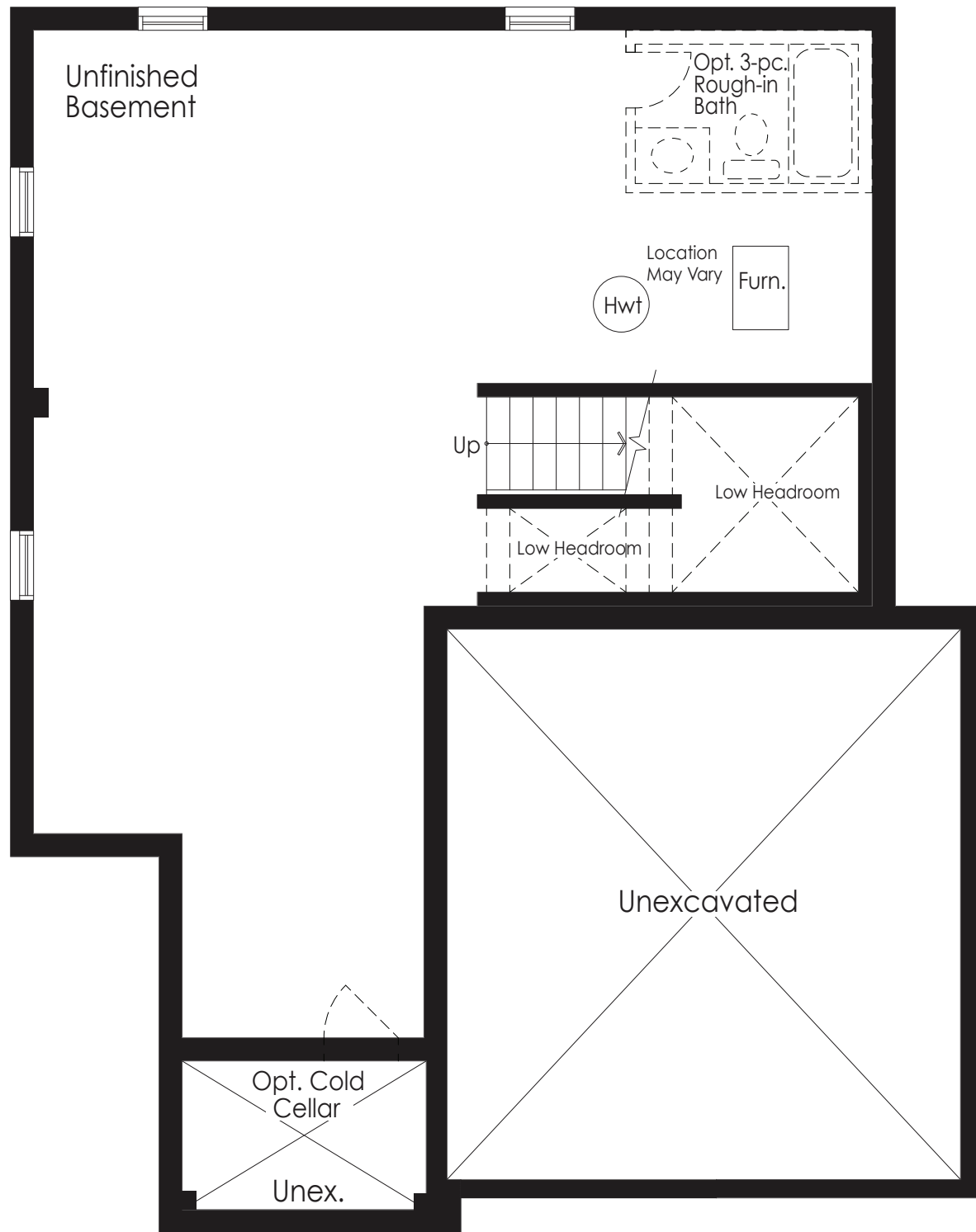
Basement Elev. A & B
