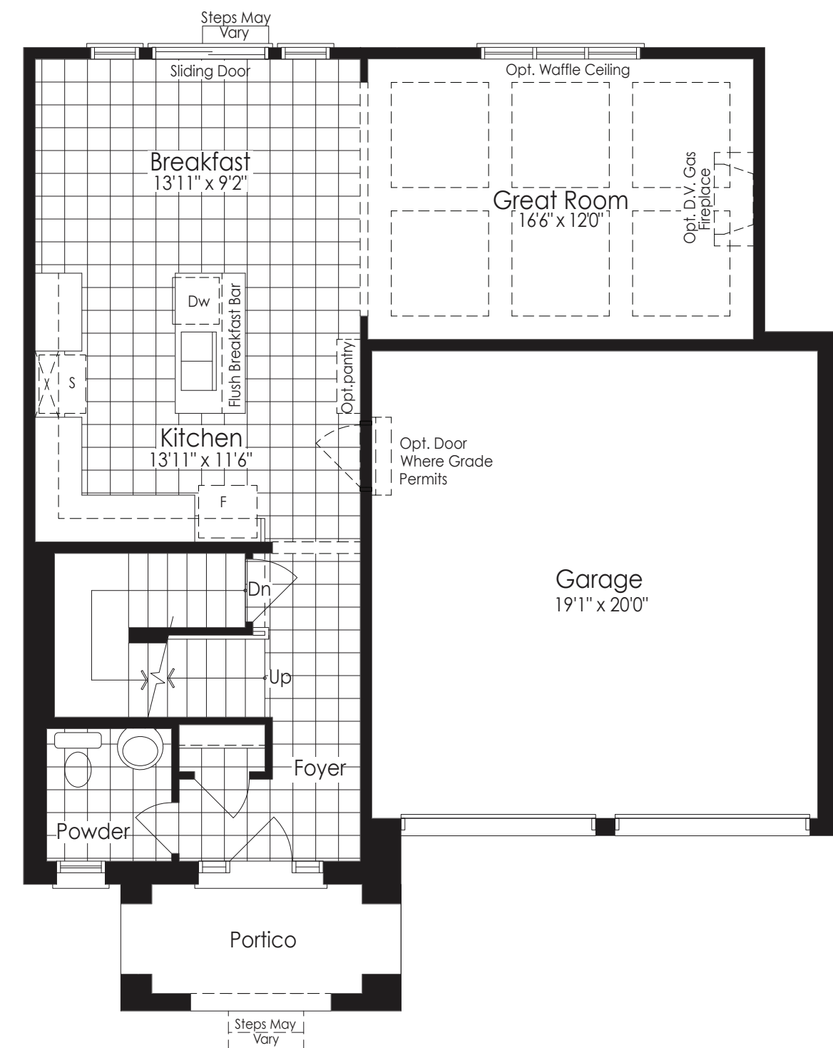
Ground Floor Elev. A & B
