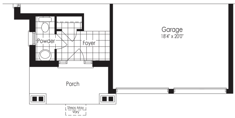
Ground Floor Elev. C
