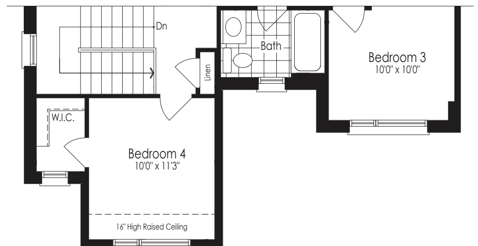
Second Floor Elev. C
