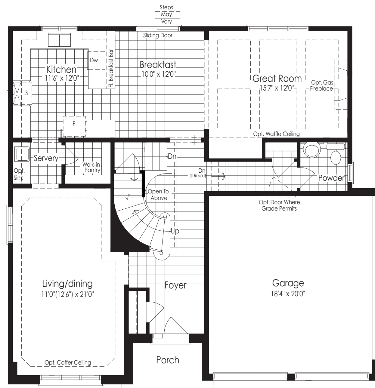
Ground Floor A
