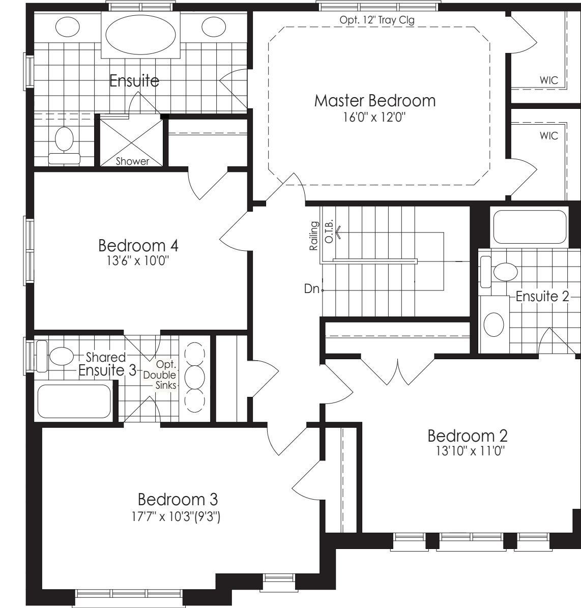
Second Floor Elev. A & B
