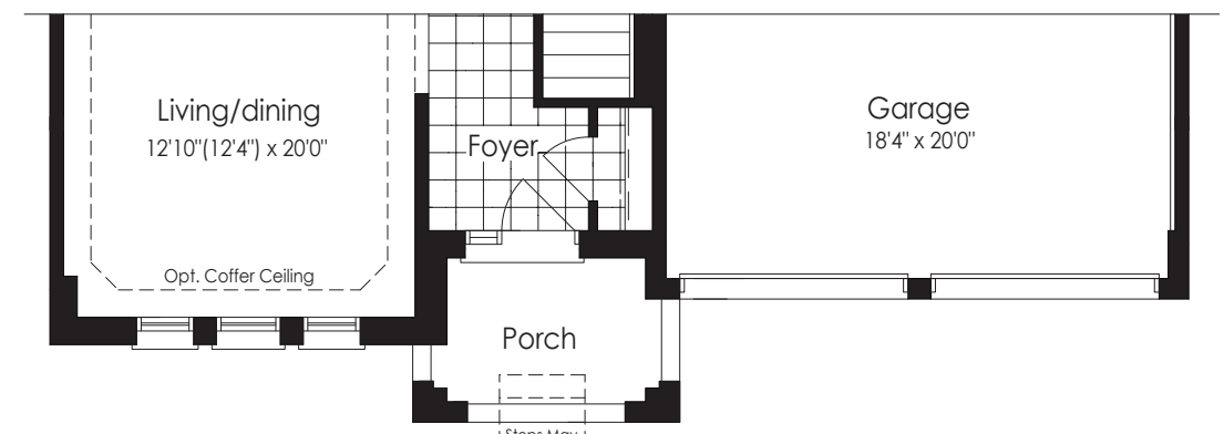
Ground Floor Elev. B
