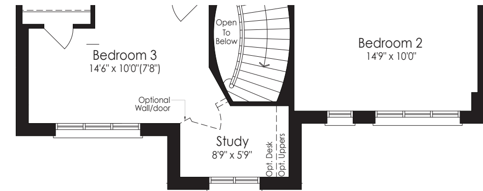
Second Floor Elev. B
