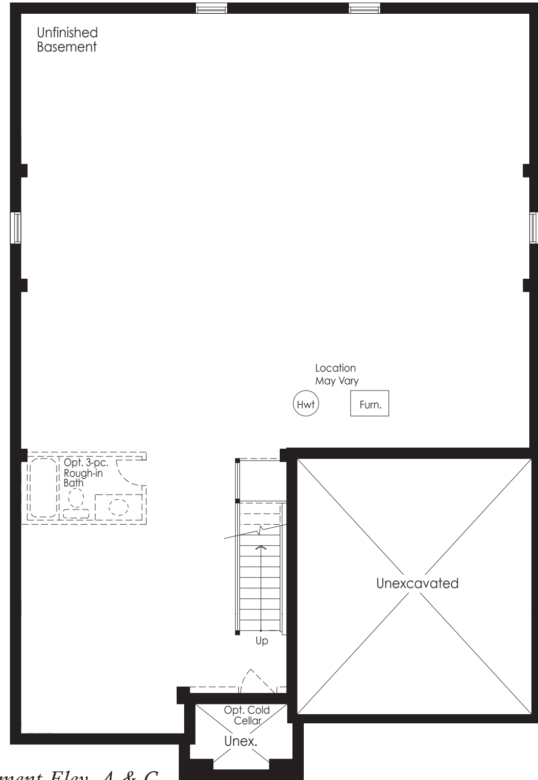
Basement Elev. A & C
