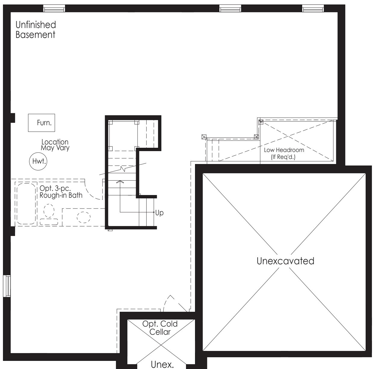
Basement Elev. A
