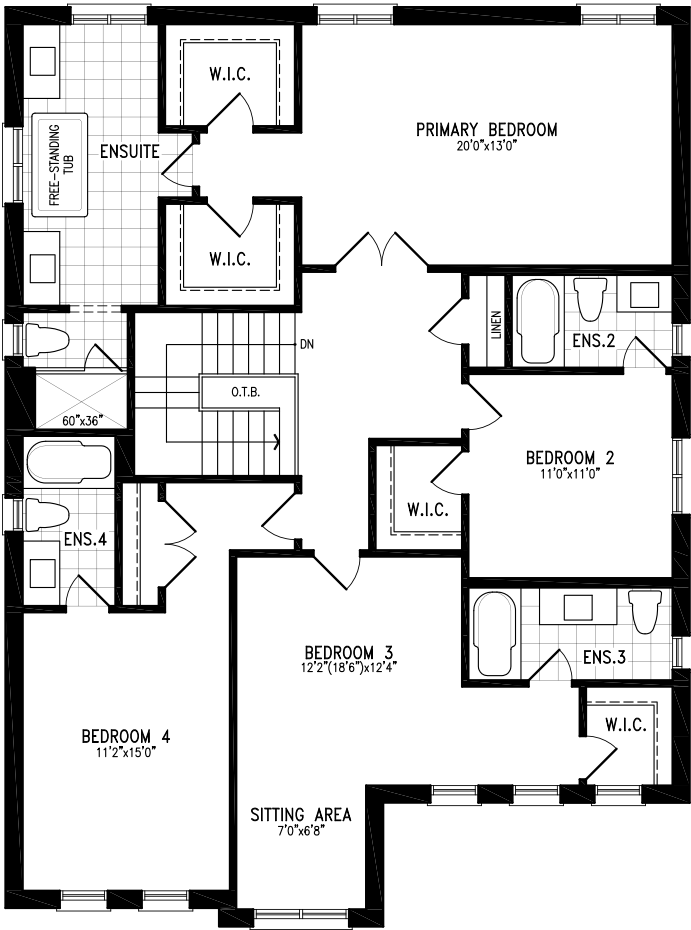
ELEVATION C SECOND FLOOR (STD. 4 BED)
