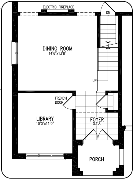
ELEVATION A GROUND FLOOR
